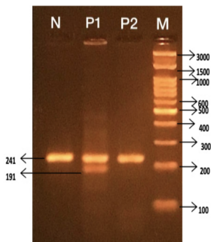
Fig 2b. The Result of Digestion of PCR Products for \beta -catenin gene fragments using EcoR1 restriction enzyme.
